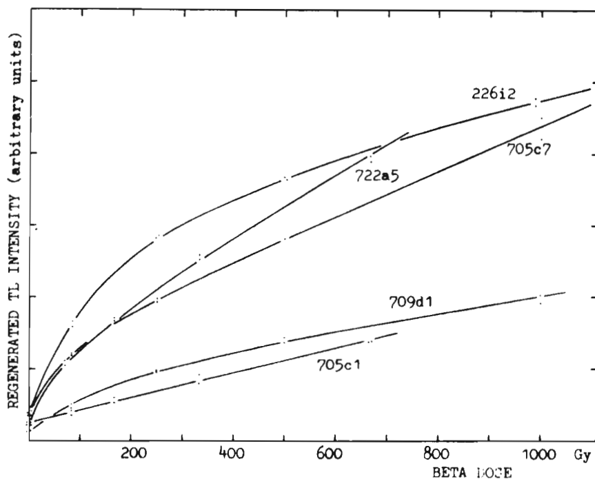
Figure 1: Growth curves at 300\text{--}310^{\circ}\text{C} regenerated by beta irradiation after 16 hours bleaching under an Oriel simulated sunlight source. Polyminerall fine grains samples on Al discs were observed with a quartz windowed EM1 9635 photomultiplier tube fitted with a Schott 2 mm thick UG11 filter. Heating rate was 2.5^{\circ}\text{C/s} . Curves are labelled with sample identifiers (Oxford Lab. refs.); 226i2, Pontnewydd Cave, N. Wales, expected age > 200\text{ka} ; 722a5, Achenheim, E. France, \sim 150\text{ka} ; 705c7, Muleta Cave, Majorca, \sim 70\text{ka} ; 709d1, Cagny-la-Garenne, N. France, \sim 400\text{ka} ; 705 c1, Muleta Cave, Majorca, \sim 50\text{ka} .
