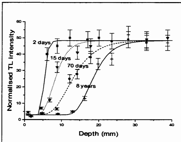
Figure 3. Thermoluminescence versus distance from the marble surface for various exposure times (Pentelikon marble). TL intensities are normalised with the second glow.
