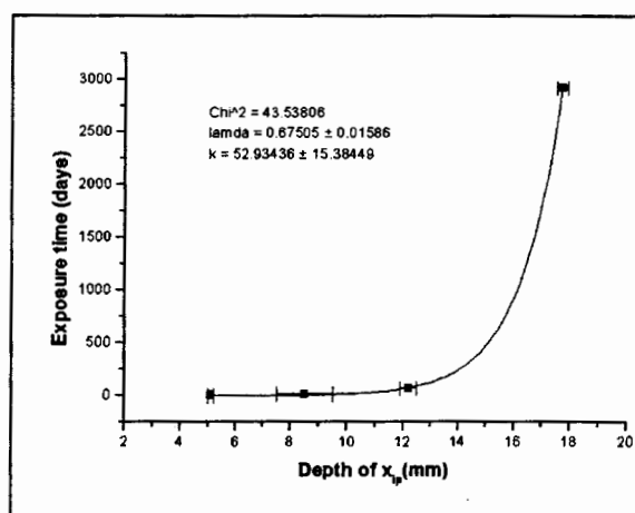
Figure 4. Time - Depth model for Pentelic marble ( x_{ip} is the inflection point of eq. (6), \lambda_0 and k as in eq. (8))
