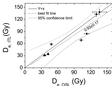
Figure 6: Comparison between D_e values derived using OSL and ITL signal at 320°C from quartz in some young samples.
