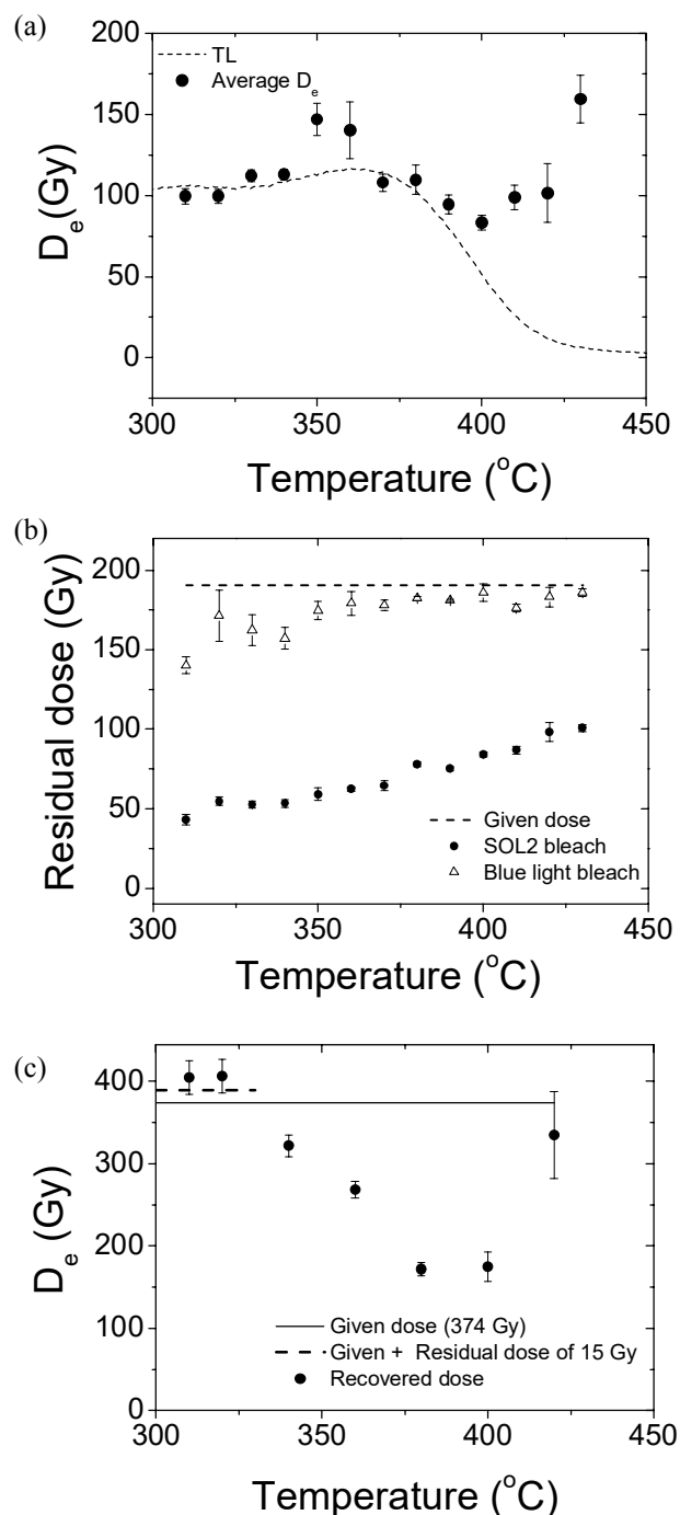
Figure 5: a) D_e values as a function of ITL measurement temperature for sample K-VII/2B. A scaled TL curve from the sample is also plotted to show the high temperature TL peaks. b) Residual dose after blue light or solar simulator bleaching for ITL signals measured at different temperatures. Same aliquots as those in (a) were used for the assessment of bleaching under these two light conditions. c) Dose recovery on previously unheated aliquots of the sample K-VII/2B as a function of ITL stimulation temperature.
