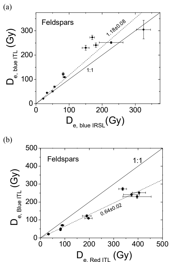
Figure 9: a) A comparison of D_e values derived using ITL at 310°C with those using IRSL from feldspars. Both the signals have been detected using the blue emission. b) A comparison between D_e values derived using the blue and red ITL signals measured at 310°C.
