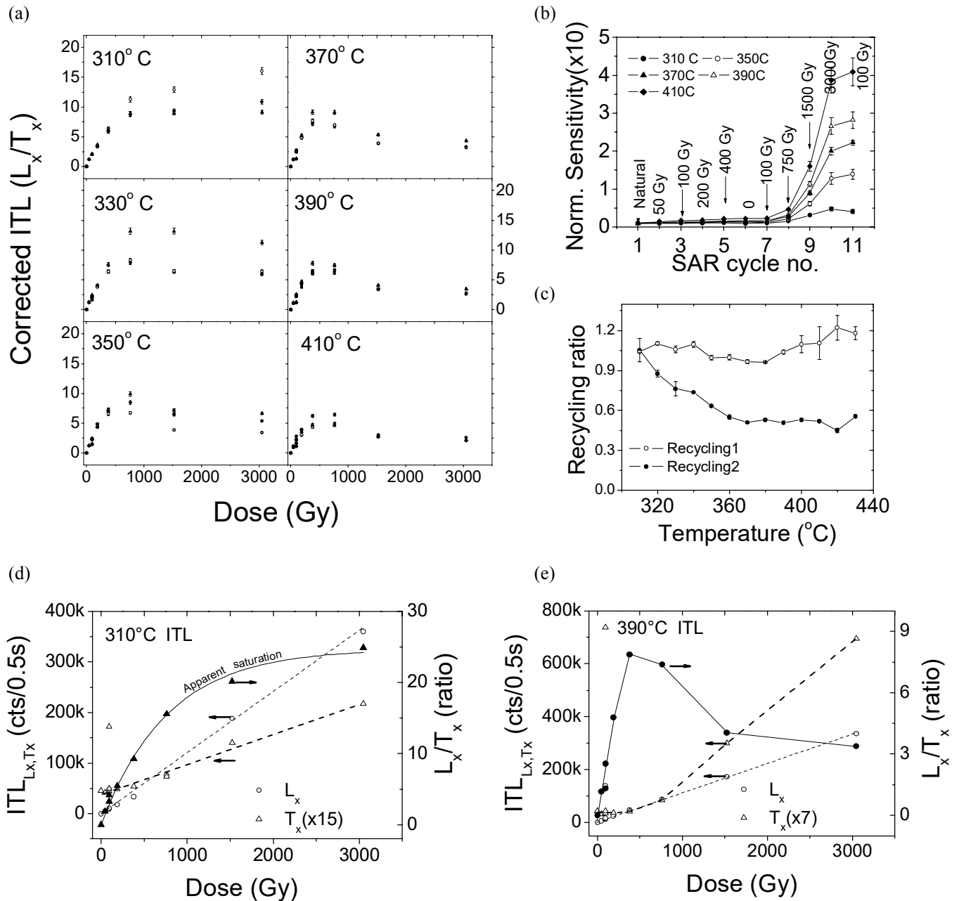
Figure 4: a) SAR dose-response curves for some representative ITL measurement temperatures. Three aliquots of the sample K-VII/2B were measured at each temperature. b) Normalised test dose response (with respect to the first value) as a function of SAR cycle or the corresponding regeneration dose (Gy). c) Recycling ratios calculated for the given 100 Gy regeneration doses. Recycling1 = ITL_{\text{cycle } 7}/ITL_{\text{cycle } 3} and Recycling2 = ITL_{\text{cycle } 11}/ITL_{\text{cycle } 7} . d) L_x , T_x and L_x/T_x ratio derived from the 310°C ITL signal and plotted as a function of regeneration dose. The T_x signal has been increased by a factor of 15 so as to match the L_x signal at 750 Gy. e) L_x , T_x and L_x/T_x ratio derived from the 390°C ITL signal and plotted as a function of regeneration dose. The T_x signal has been increased by a factor of 7 so as to match the L_x signal at 750 Gy.
