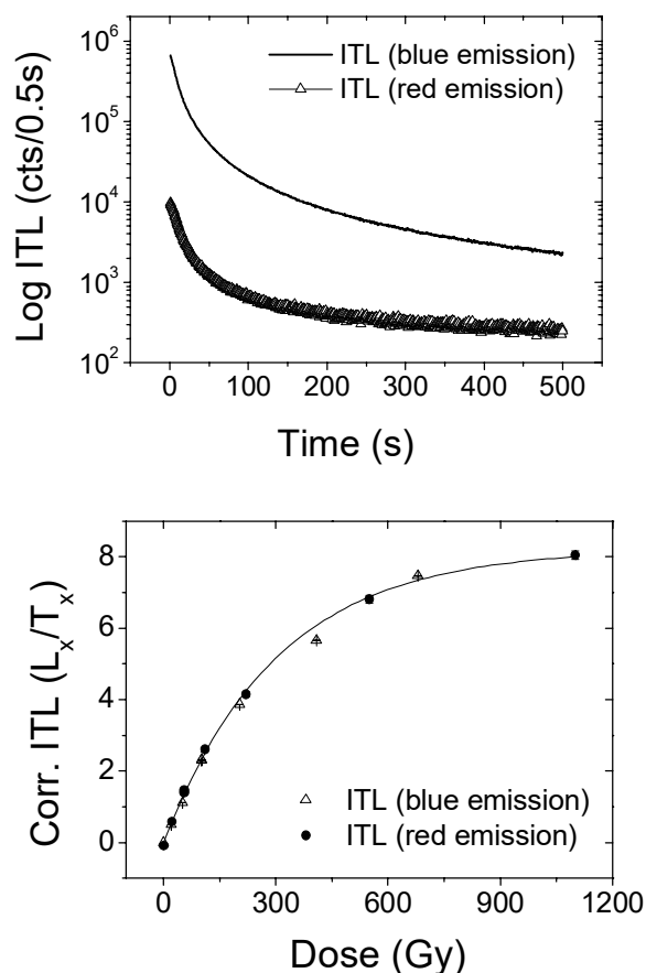
Figure 7: a) Blue and red emission ITL decay curves at 310°C measured from sample K-IX/49. The data is plotted on a log ITL scale. b) SAR dose response curves using blue and red ITL at 310°C.
