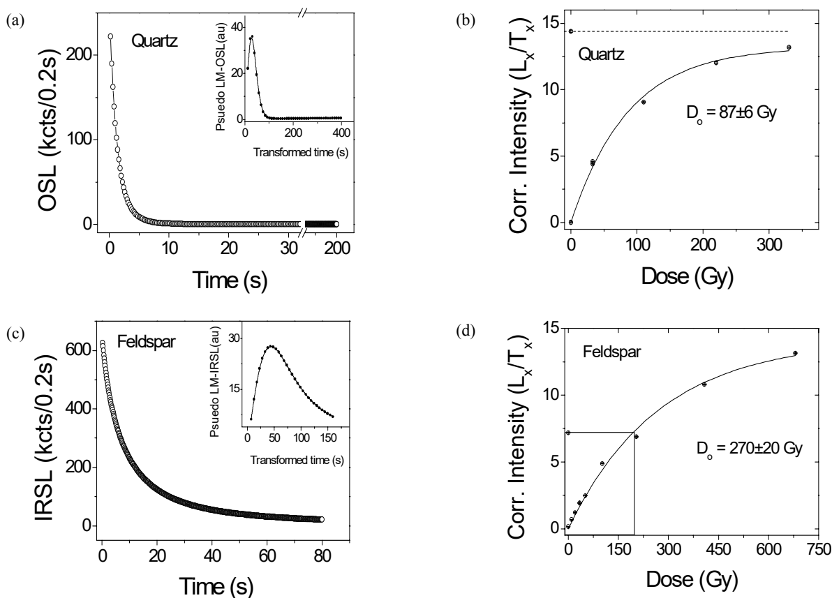
Figure 1: a) Natural OSL decay curve from a quartz aliquot of sample K-IX/49. The inset shows a pseudo LM-OSL curve derived from the same data. b) Dose response curve for the same aliquot of quartz. c) Natural IRSL decay curve from a feldspar aliquot of sample K-IX/49. The inset shows a pseudo LM-IRSL curve. d) Dose response curve for the same feldspar aliquot. The first 0.8s was used for signal integration in both IRSL and OSL decay curves.
