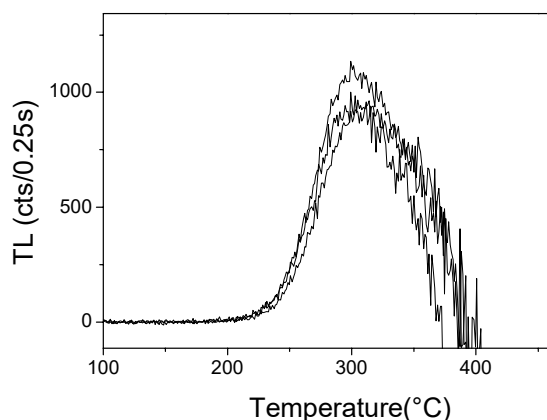
Figure 8: Background subtracted red emission TL signal from three aliquots of the sample SNG1 containing natural dose. A heating rate of 2°C/s was used.
