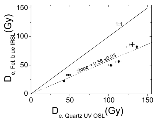
Figure 2: A comparison of dose estimates derived using Quartz OSL (UV emission) and Feldspar IRSL (blue emission).
