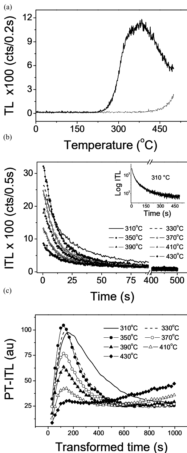
Figure 3: a) TL peak of an aliquot of quartz from a modern sample (BTh0) after a dose of 34 Gy and a preheat of 260°C for 10s. TL was measured at the rate of 5°C/s. The dotted curve is the repeat TL run after the TL signal had been measured. b) Natural isothermal TL decay curves measured at different temperatures c) same data plotted as peak transformed isothermal TL (PT-ITL) curves.
