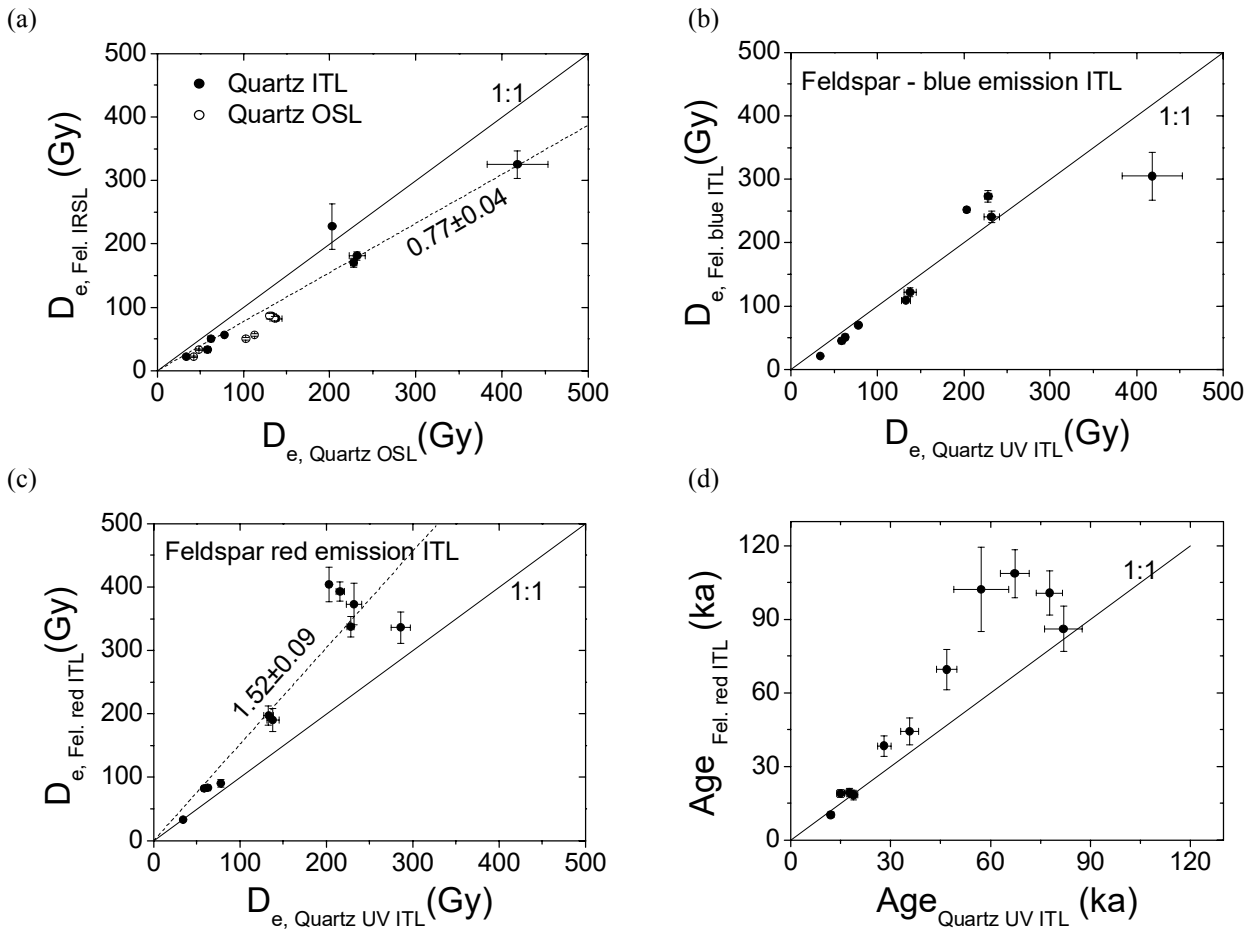
Figure 10: a) A comparison between D_e values derived using IRSL from feldspars, and OSL and 320°C ITL signals from quartz. b) A comparison between D_e values derived using blue emission ITL at 310°C from feldspars and UV emission ITL at 320°C from quartz. c) A comparison between D_e values derived using red emission ITL at 310°C from feldspars and UV emission ITL at 320°C from quartz. d) A comparison between feldspar red ITL and quartz ITL ages (same D_e data as (c)).
