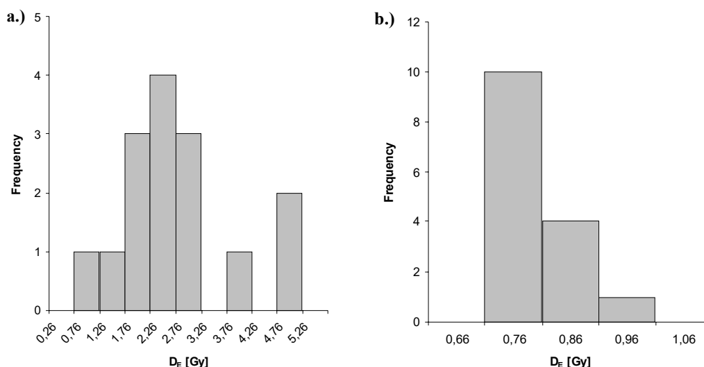
Figure 3: Examples of typical dose distributions from coarse- (RW3, figure a) and fine-grain (EL5, figure b) quartz samples. Due to the small number of grains on the coarse grain aliquots (ca. 500) the distribution is much broader than that of the fine grain aliquots which have ca. 14,000 grains per aliquot.
