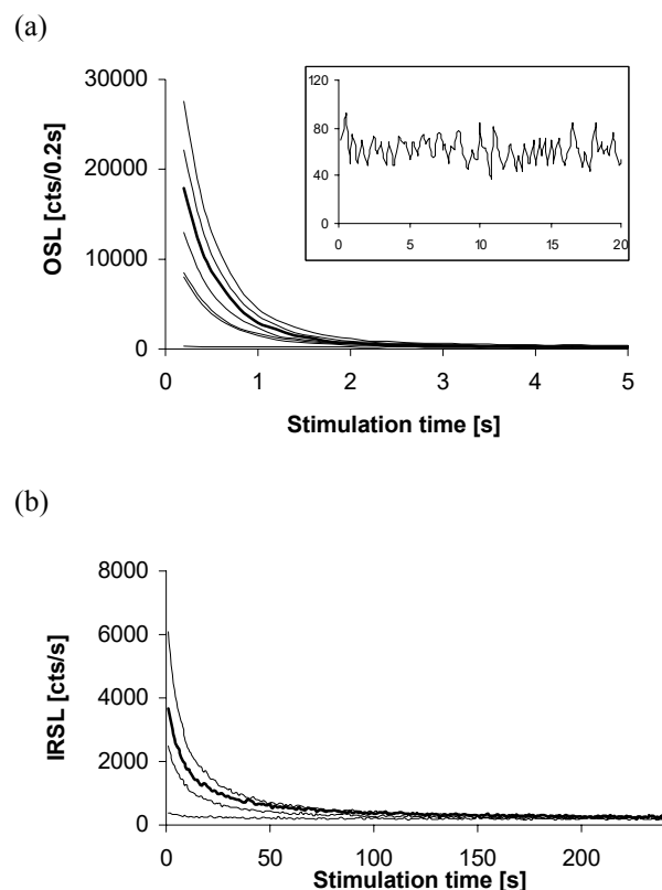
Figure 2: OSL and IRSL decay curves for sample EL5 (figure a: quartz fine grains; figure b: polymineral fine grains). The graphs show the decay curves of the natural signal (bold line) and the regenerated signals. Inset of figure a: IRSL stimulated signal of the quartz fine grain fraction. The sample shows no IRSL signal, thus no feldspar contamination (for axis labels see large figure).
