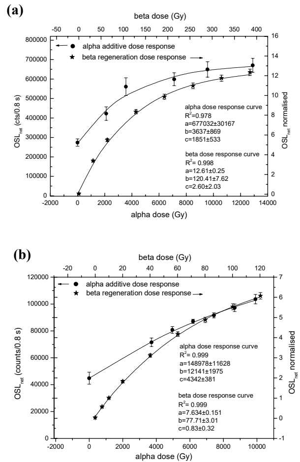
Figure 1: Alpha- and beta dose response curves of two samples fitted to the equation y = a \times (1 - e^{-\frac{x+b}{c}}) . Each alpha dose point is based on the mean and standard deviation of 3 aliquots after normalisation to the natural OSL. The beta dose points are derived from a SAR measurement of one aliquot. (a) Sample exhibiting a very high natural dose (LV184); (b) sample exhibiting a high natural dose (LV05)
