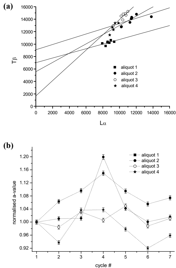
Figure 3: Results from the sensitivity change test shown by sample LV06. Data were obtained using the protocol described in Figure 2, but using repeated alpha doses. An alpha regeneration dose of \sim 90 Gy was administered for 7 cycles (beta test dose was \sim 4 Gy). (a) Plot of T_\beta versus L_\alpha ; linear fitting was applied to the data set of each aliquot. (b) the a-values of the 4 aliquots of each alpha regeneration cycle normalised to the a-value of the first cycle.
