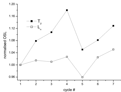
Figure 4: Detail of the sensitivity test illustrated in Figure 3(a). L_\alpha and T_\beta of aliquot 1 (LV06), normalised to the first cycle are plotted separately against cycle number.
