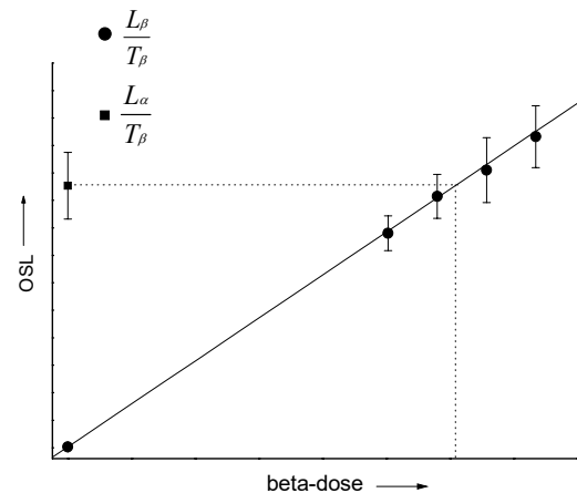
Figure 2: SAR protocol designed to determine the a-value. The a-value results from the projection of L_\alpha/T_\beta onto the beta dose response curve obtained from a standard SAR protocol. For details see text.
