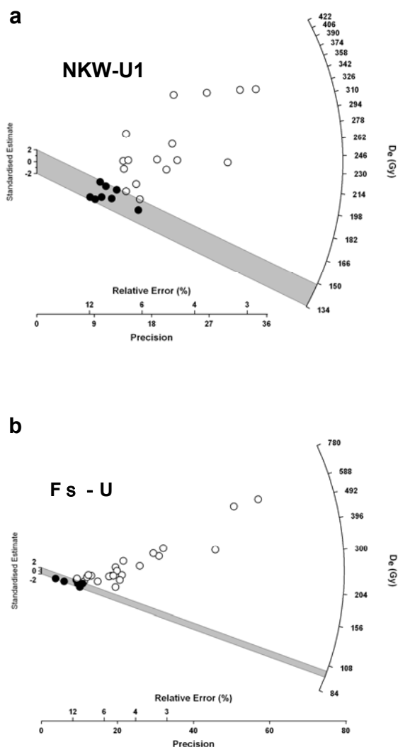
Figure 7: D_e values of the terrace deposits (corresponding to the deposition age) of NKW-U1 (a) and Fs-U (b), as calculated from divided fragments from single grains (filled circles) within the 2\sigma range of the radial plot.
