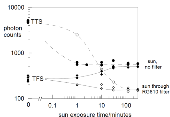
Figure 1: Reproduction of data presented in Figure 11 of Huntley and Clague (1996), showing the effect of a prior light exposure on the luminescence intensity due to 1.4 eV excitation. Aliquots of a 300-year-old tsunami sand (TTS) and of a zero-age source sand (TFS) were exposed to unfiltered (solid symbols) and filtered (open symbols) sunlight. No preheat was used.
