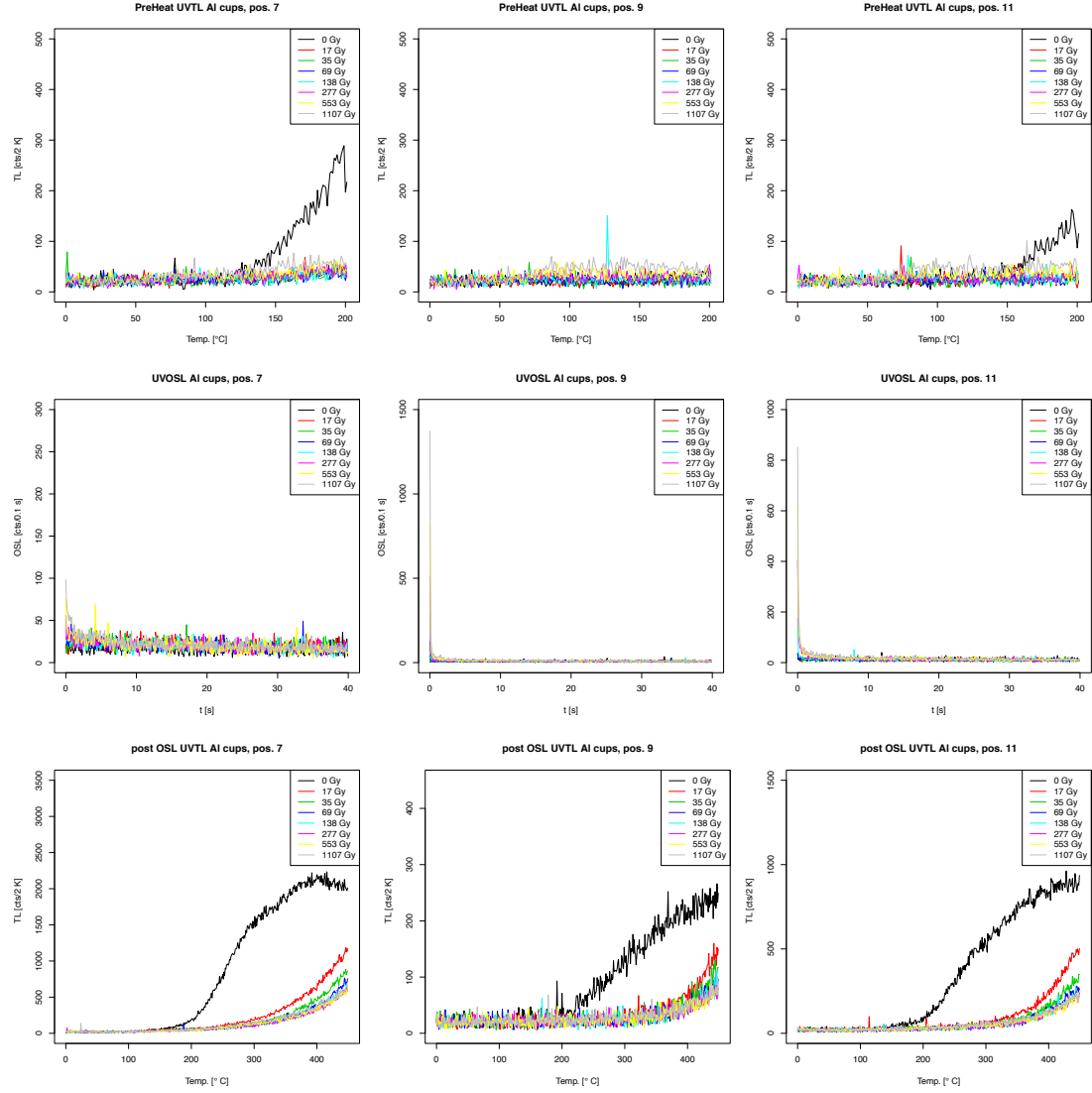
Figure 7: The natural and regenerated BOSL signals, detected in the UV window, were recorded for 3 Al cups at 125 °C for 40 s (middle row). The measurements included a preheat step (200 °C for 10 s, upper row) before and a final TL measurement up to 430 °C after OSL readout to detect photo-transferred and optically unbleachable signal contributions (lower row). The cups were \beta -dosed up to ca. 1 kGy. No N_2 was used. For \beta -doses < 500 Gy the Al cups are free from substantial BOSL signals. For higher doses, a peak in the foremost signal channels was detected.
