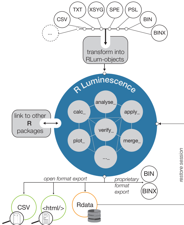
Figure 2. R ‘Luminescence’ package structure with indicated input/output interfaces. Once the raw measurement data have been transformed into an RLum -object, data can be passed without further transformation from one function to another within the package environment.
