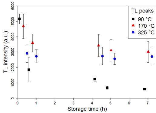
Figure 7. Intensity variation of TL peaks at 90, 170 and 325 °C (given dose of 200 Gy) from kyanite aliquots irradiated with 200 Gy and stored at room temperature for different times (storage time). Each TL intensity point is represented by the average of two aliquots. Data points are offset in the x axis to avoid points overlapping.
