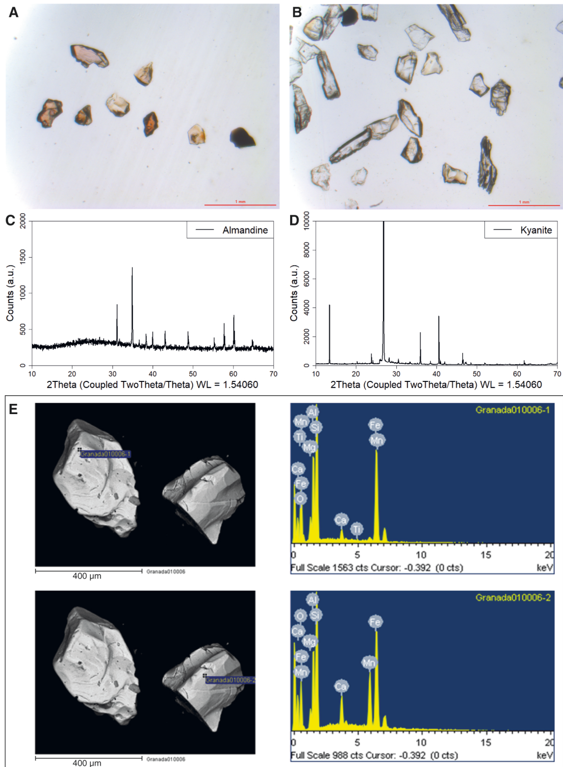
Figure 1. Almadine (A) and kyanite (B) grains under the optical microscope. XRD spectra of studied almandine (C) and kyanite (D) samples. E) Scanning electron microscope image (secondary electrons detector, left) from grains of almandine and energy dispersive spectrum (right) showing the chemical composition corresponding to the points highlighted in the images at left.
